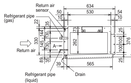
Upper View
