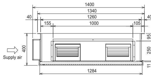
Back View
